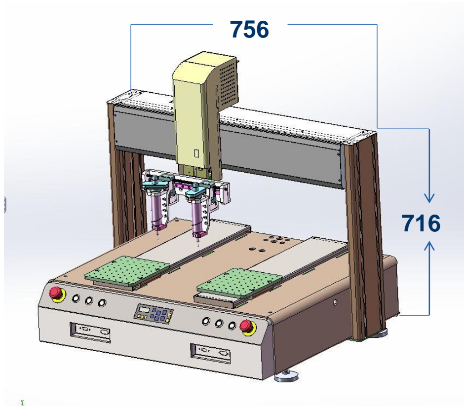
DJ-5430YY Automated Dispensing Robot
